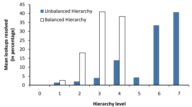
Fig. 8. Mean lookups resolved at different levels of balanced and unbalanced controller hierarchies.
