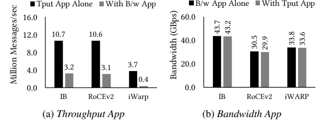
Figure 4: Throughput-sensitive application requires isolation from bandwidth-sensitive applications.
