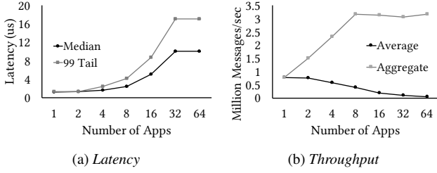
Figure 26: Latencies and throughputs of multiple latency-sensitive applications in InfiniBand. Error bars (almost invisible due to close proximity) represent the applications with the lowest and highest values.
