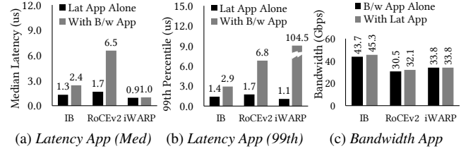
Figure 3: Latency-sensitive applications require isolation against bandwidth-sensitive applications.
