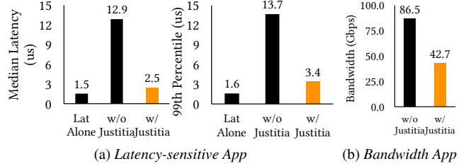
Figure 30: [100 Gbps InfiniBand] Performance isolation of a latency-sensitive application against a bandwidth-sensitive application.
