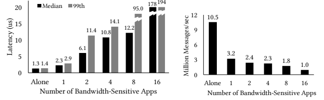
Figure 29: Impact of increasing background bandwidth-sensitive applications (sending 1MB messages) in InfiniBand.
